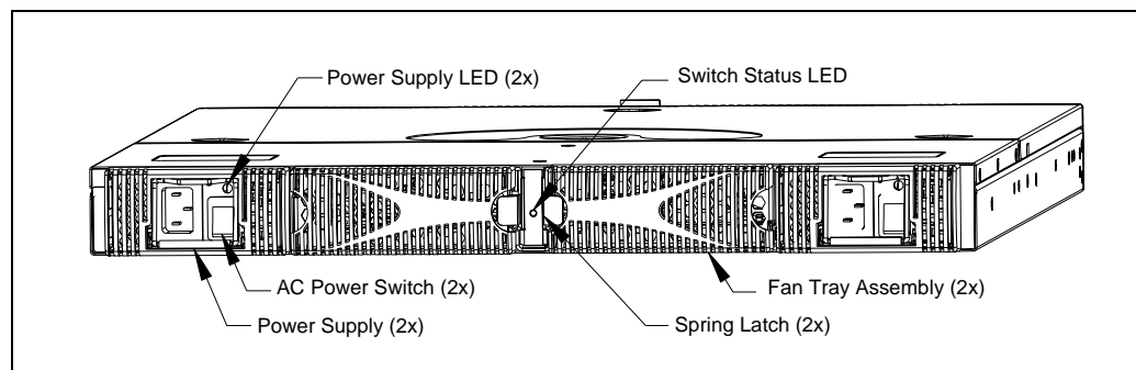
Figure 1-2 The power supply side of the FC 16B
